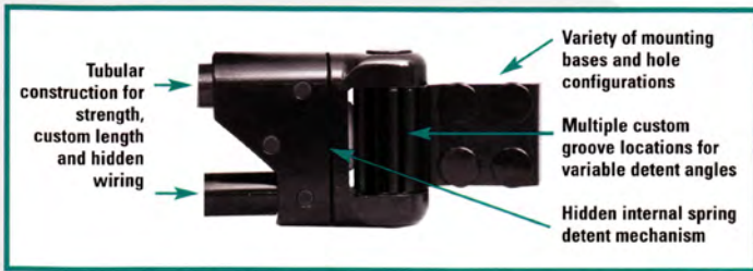
All wiring is hidden inside mirror and arm for aerodynamic styling and functionality
