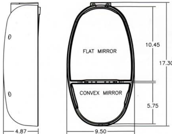
AviaStyle® passenger side, overhang mirror with Spring-Break® breakaway arm assembly.
